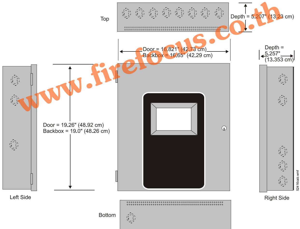
Cabinet Measurements
